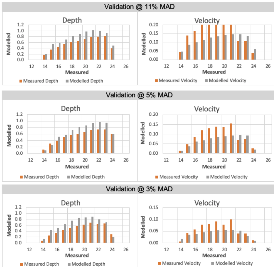
Figure 4-19. Koksilah River EFA, Validation of SEFA Model Results for Transect 4.1.
