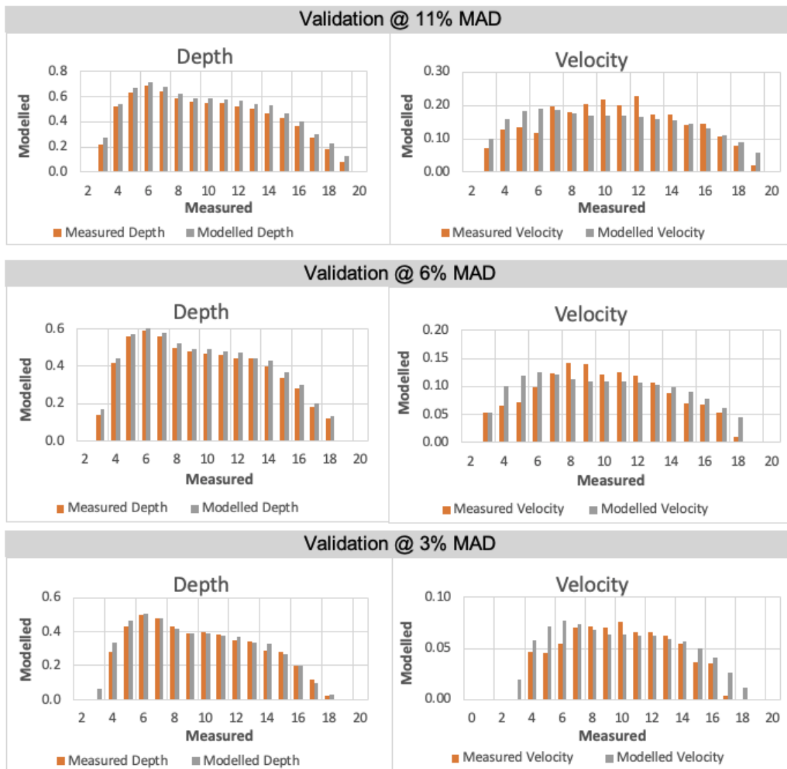
Figure 4-14 Koksilah River EFA, Validation of SEFA Model Results for Transect 1.3.
