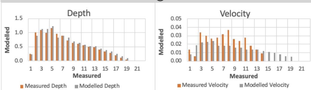
Figure 4-24. Koksilah River EFA, Validation of SEFA Model Results for Transect 5.35.
