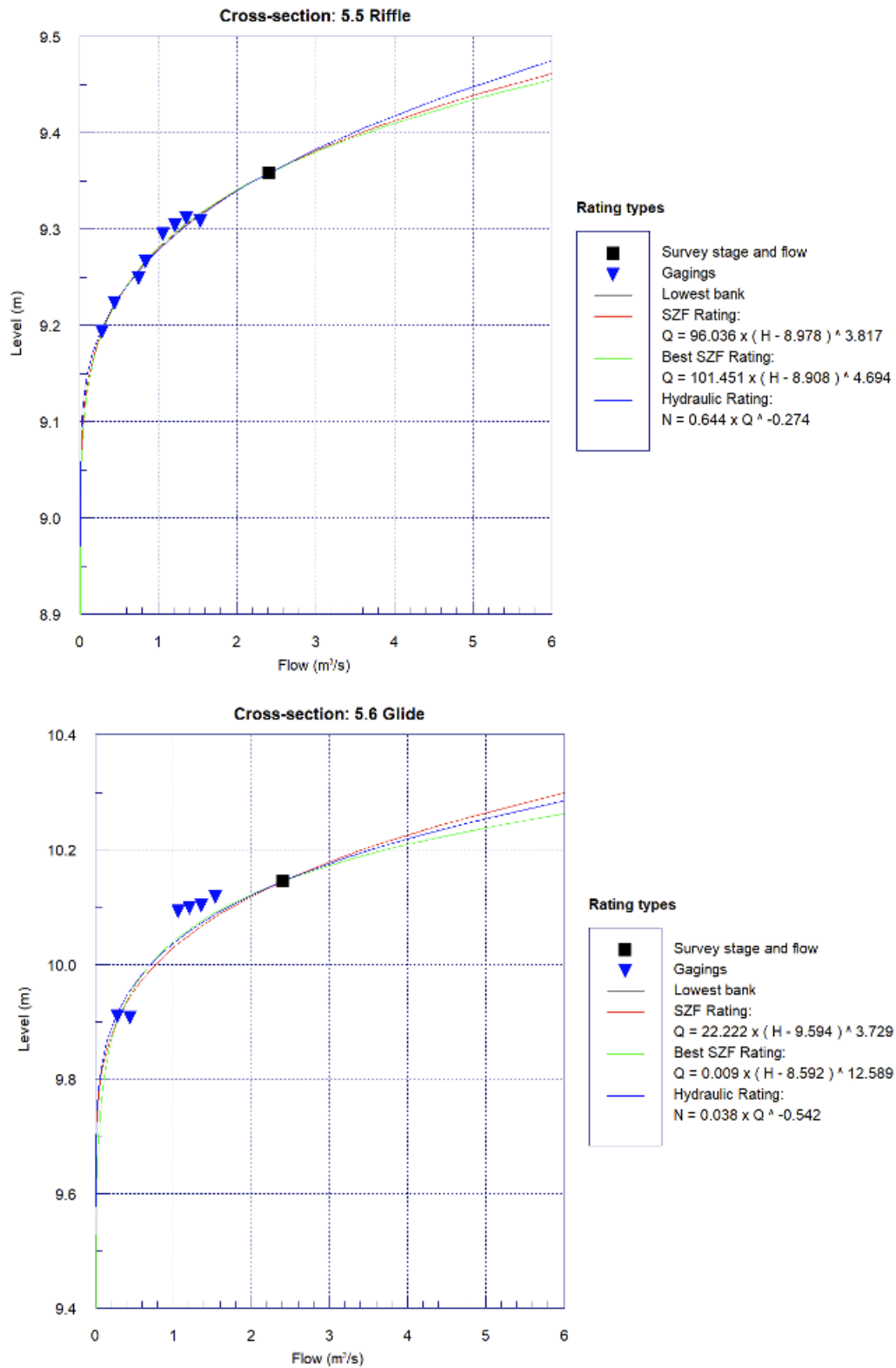
Figure 4-8. Koksilah River EFA, Rating Curves for Transects 5.5 and 5.6.
