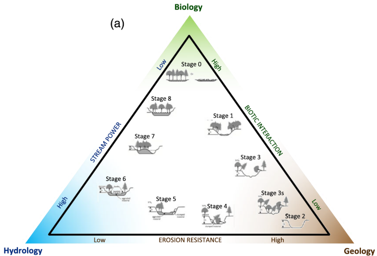
Figure 2-4. Stream Evolution Triangle (SET).
