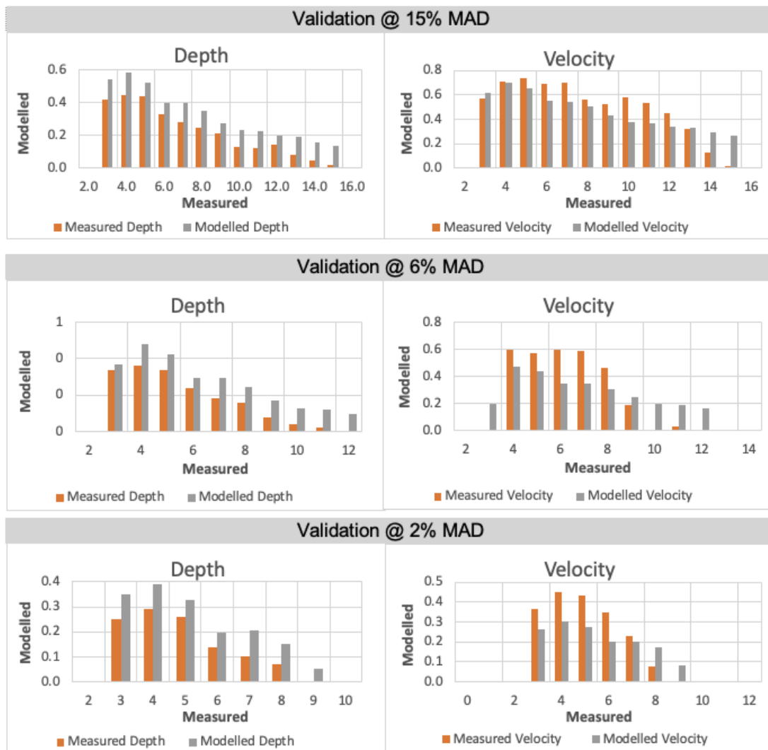
Figure 4-12. Koksilah River EFA, Validation of SEFA Model Results for Transect 1.1.
