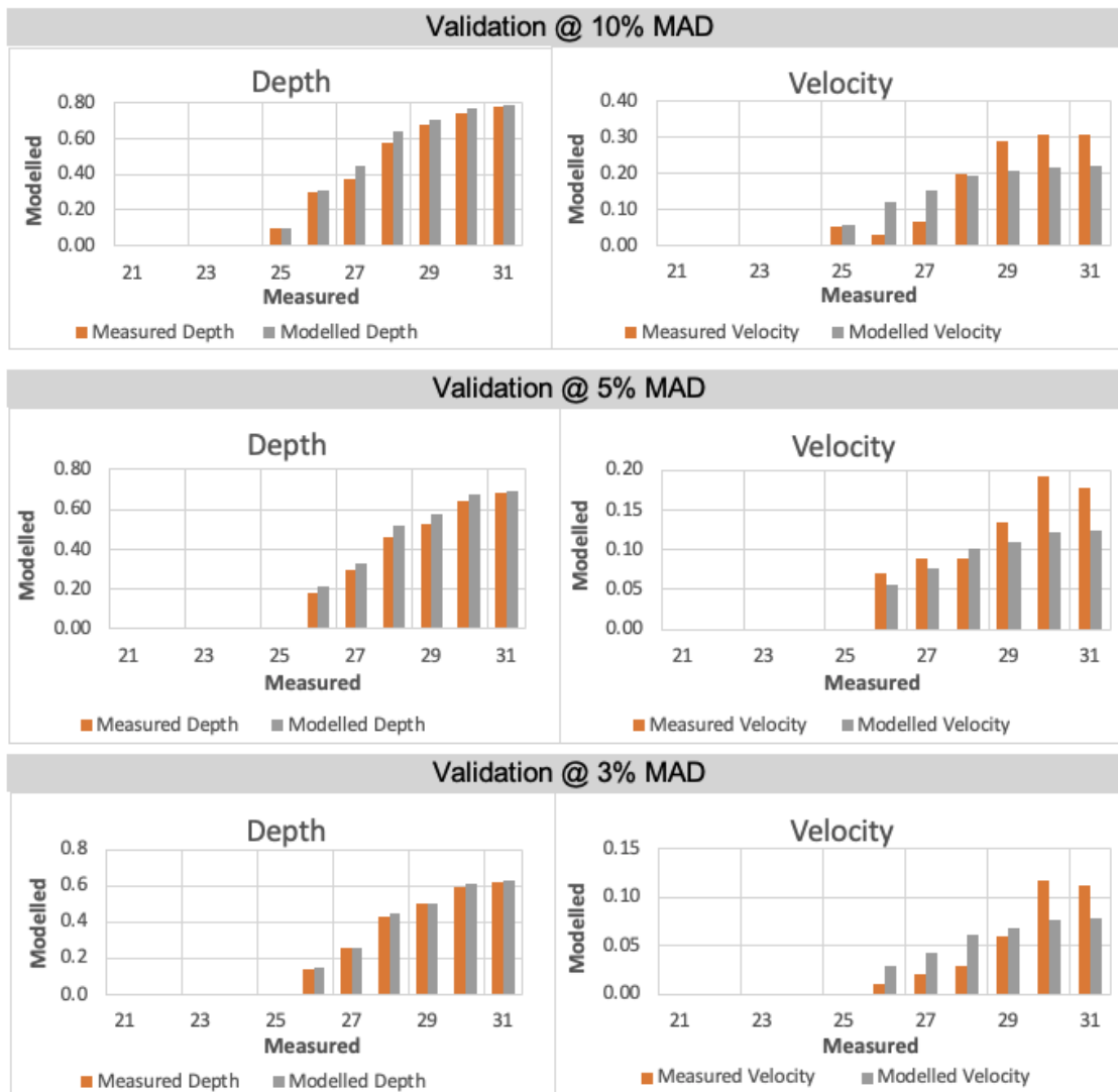
Figure 4-20. Koksilah River EFA, Validation of SEFA Model Results for Transect 4.3.
