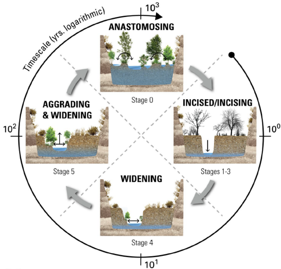
Figure 2-4. Riverscape Evolution Model (REM).
