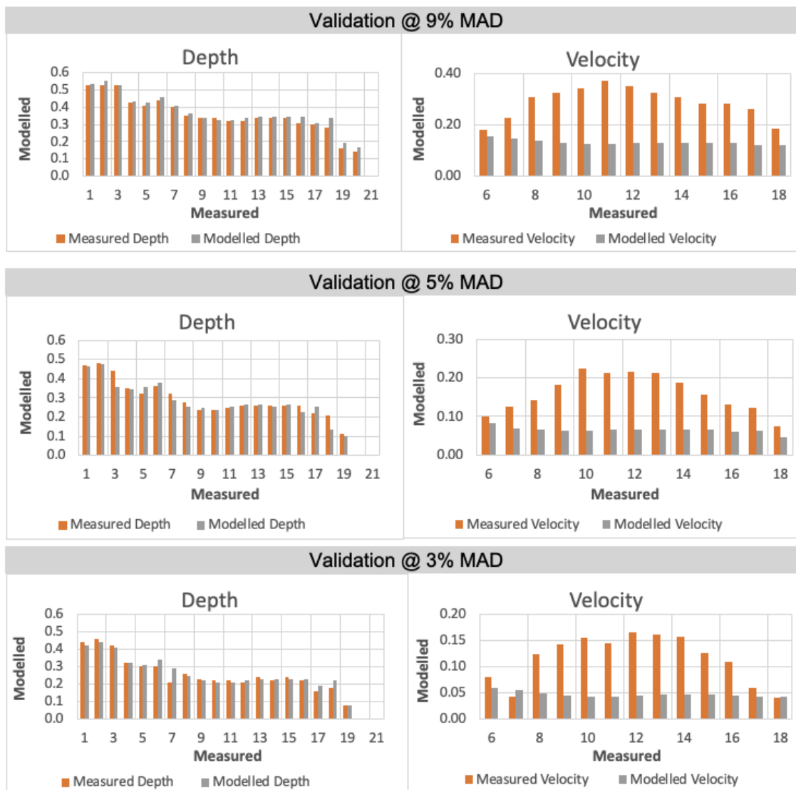
Figure 4-18. Koksilah River EFA, Validation of SEFA Model Results for Transect 3.1.
