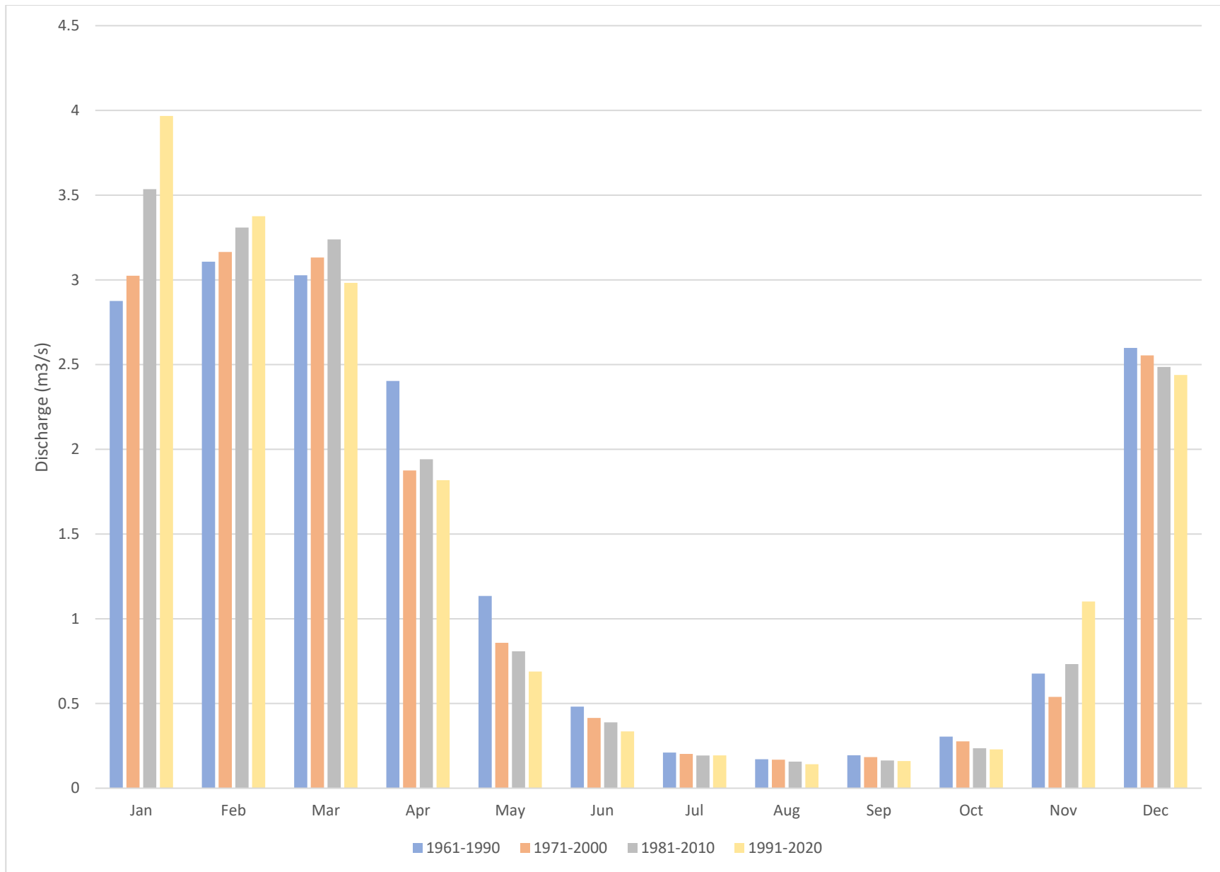
Figure 5. Koksilah River 7Q10 Discharge
