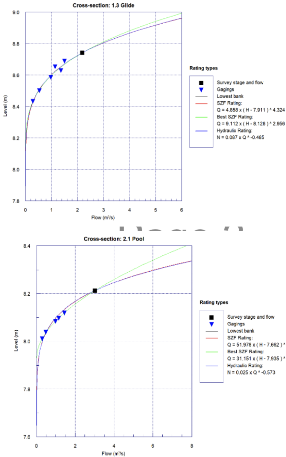
Figure 4-2. Koksilah River EFA, Rating Curves for Transects 1.3 and 2.1.
