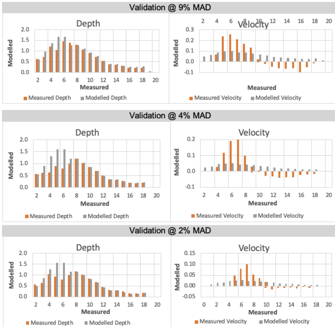
Figure 4-15. Koksilah River EFA, Validation of SEFA Model Results for Transect 2.1.
