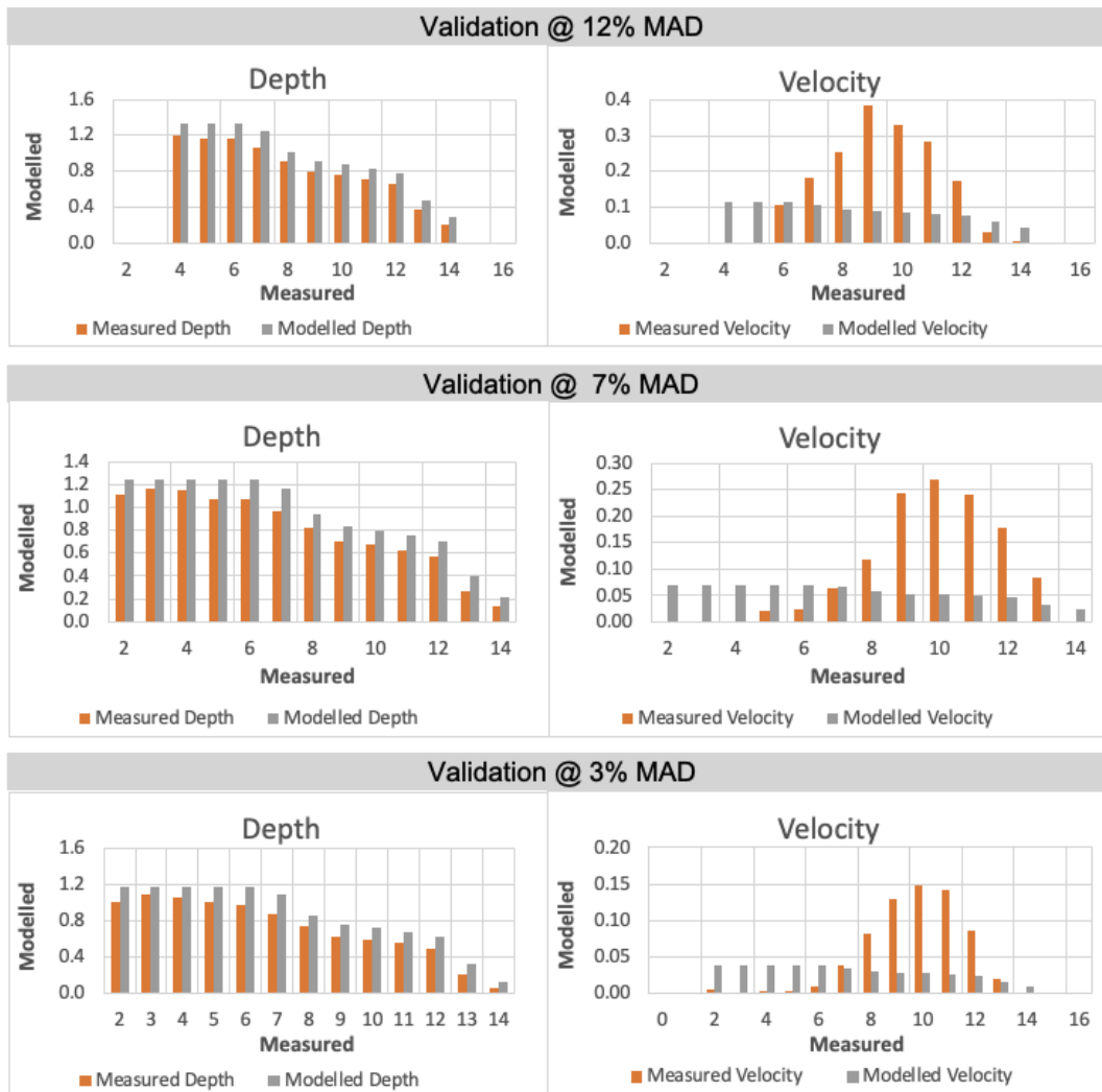
Figure 4-13. Koksilah River EFA, Validation of SEFA Model Results for Transect 1.2.
