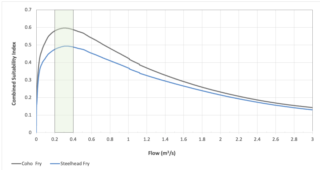
Figure 4-38. Koksilah River EFA, Area Combined Suitability Index for Shallow Glides.
